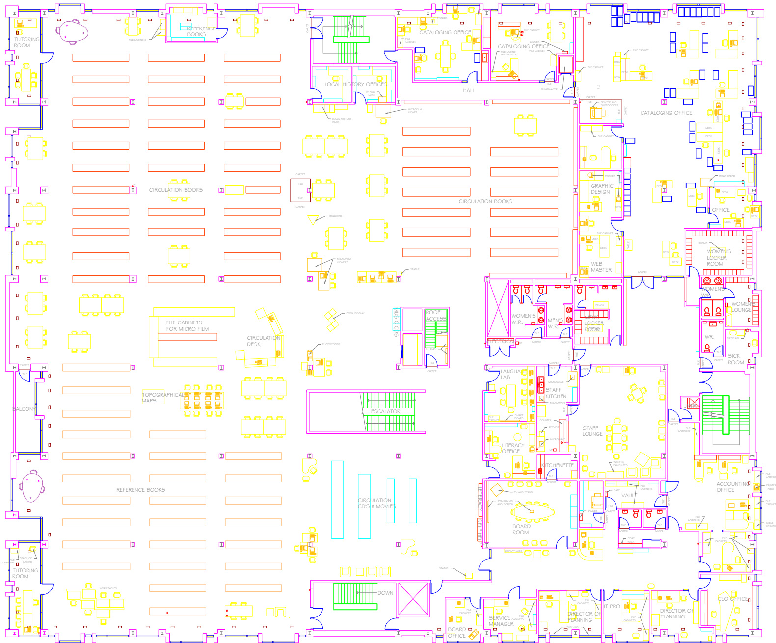
CENTRAL SECOND FLOOR PLAN
